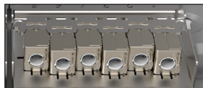
ZTB Modular array With Cat6A STP Keystone Jacks
