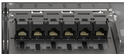
ZTB Modular array With Cat6 UTP Keystone Jacks – Various colours
