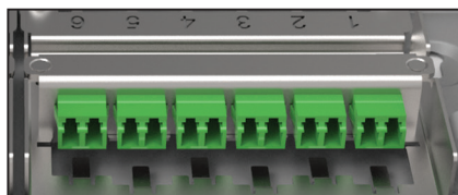
ZTB Modular array with LC Duplex adaptors – Available in SM, SM APC, OM3, OM4, OM5
