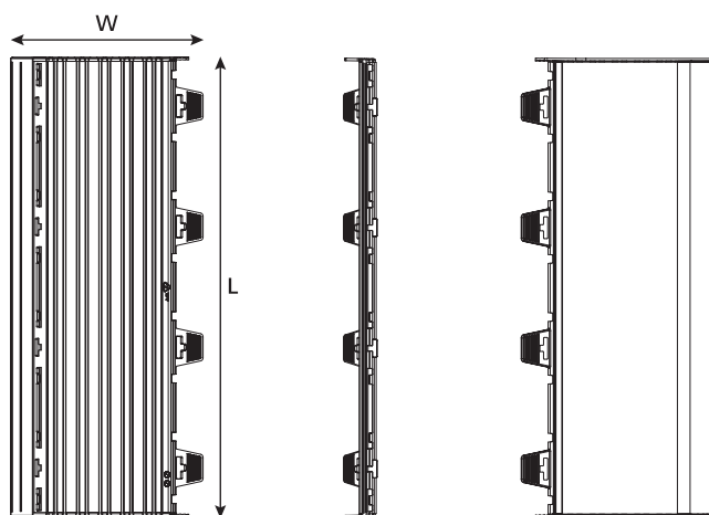
External View
