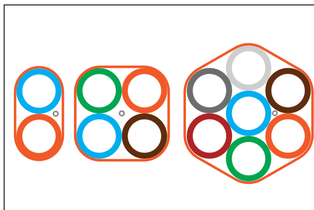
Microduct Bundles 14/10mm.
