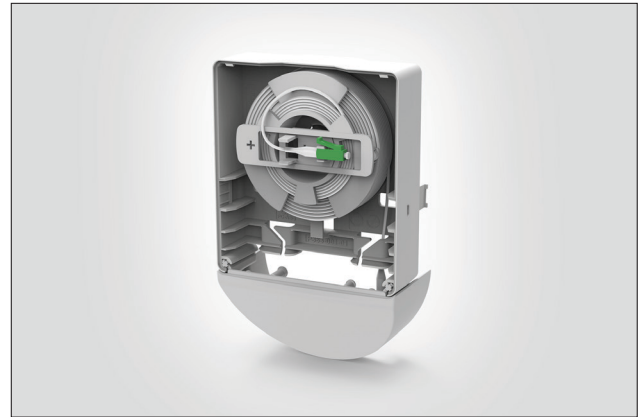
Internal view of the FWO Extension Module with fibre spool, LC/APC SX connectors.
