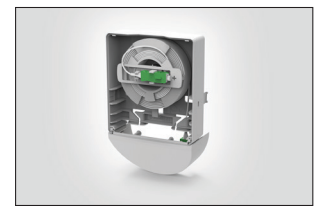
Internal view of the FWO Extension Module with fibre spool, SC/APC SX connectors.
