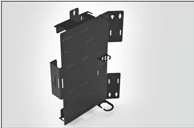
MB-AFN/FFE-PB001 Mounting Bracket.
