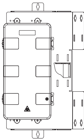
Front View shown with Aerial Fibre Node
