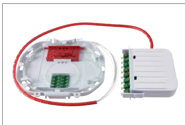
Splitter Assembly
